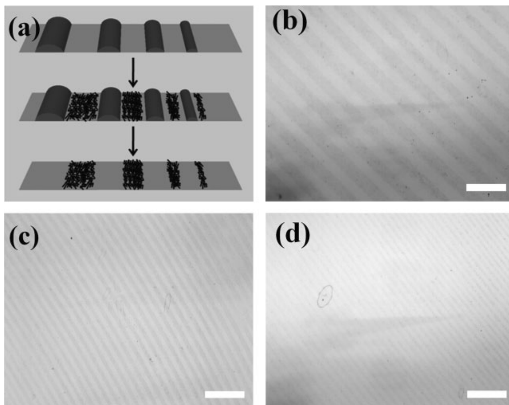
Figure 3. a) Schematic stepwise representation of formation of gradient concentric MWNT rings. Evaporation-induced self-assembly of MEH-PPV rings on Si substrate from MEH-PPV toluene solution in sphere-on-flat geometry, showing a decrease in \lambda_{C-C} and height of the rings, h , from outermost ring (left) toward the original sphere/Si contact center (right) (first panel). Then a drop of MWNT/PDDA water solution was drop-cast onto the MEH-PPV ring-patterned Si substrate. Upon completion of water evaporation, MWNT rings were formed in between MEH-PPV rings (second panel). After selective removal of MEH-PPV with toluene, gradient concentric MWNT rings can be revealed (last panel). b)–d) Optical micrographs of highly ordered, gradient MWNT rings on Si substrate over large areas produced by template-assisted self-assembly as described in (a) ( Method a ). The locations of MWNT rings corresponding to original MEH-PPV templates are (a) at X_1 , (b) at X_2 , and (c) at X_3 (Fig. 1b), respectively. Scale bars = 45 \mu\text{m} .
