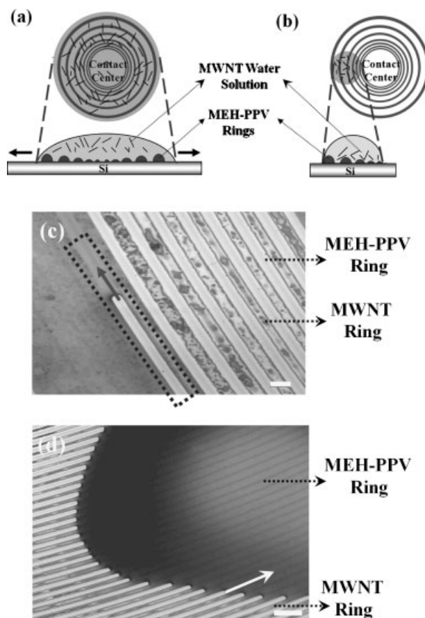
Figure 2. a) and b) Methods used to cast the MWNT/PDDA water solution ( c = 0.05 \text{ mg ml}^{-1} ). (a) Solution overspread the entire surface of ring patterns ( Method a ). (b) Solution covered only a small part of ring pattern ( Method b ). (c) Optical micrograph during the formation of MWNT rings by Method a . The water meniscus retreated along the MEH-PPV ring surface (i.e., dewetting on hydrophobic MEH-PPV ring), as indicated by an arrow in a dashed box, thereby forming two MWNT rings adjacent to each other. Scale bar = 30 \mu\text{m} . d) Optical micrograph during the formation of MWNT rings by Method b . The solution was confined within the MEH-PPV rings. As water evaporated (direction indicated by an arrow), a periodic family of MWNT rings were left behind on the Si substrate. Scale bar = 70 \mu\text{m} .
